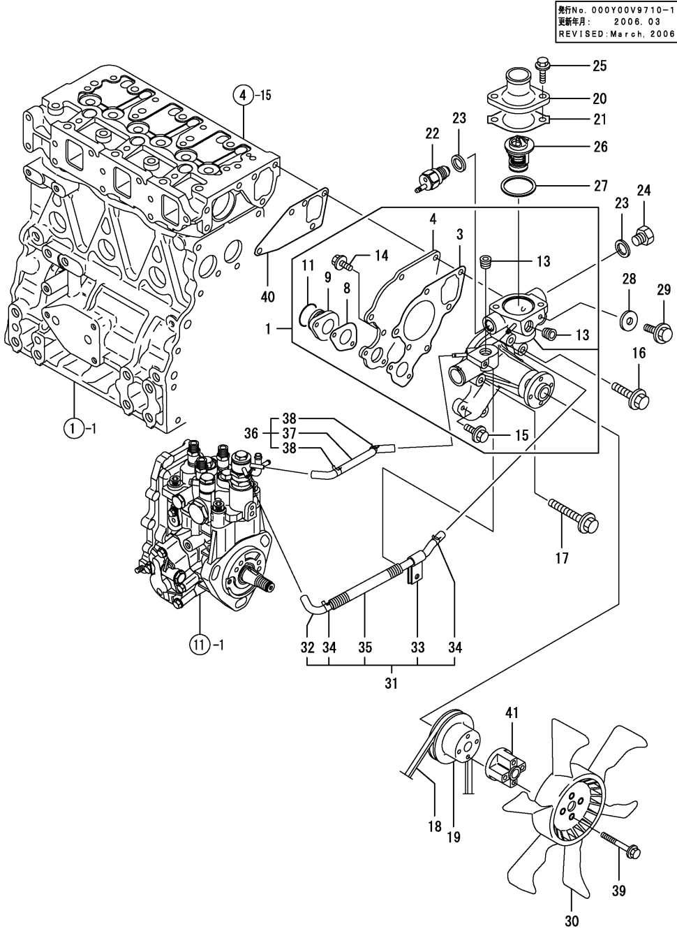
Fig.10.COOLING WATER SYSTEM
