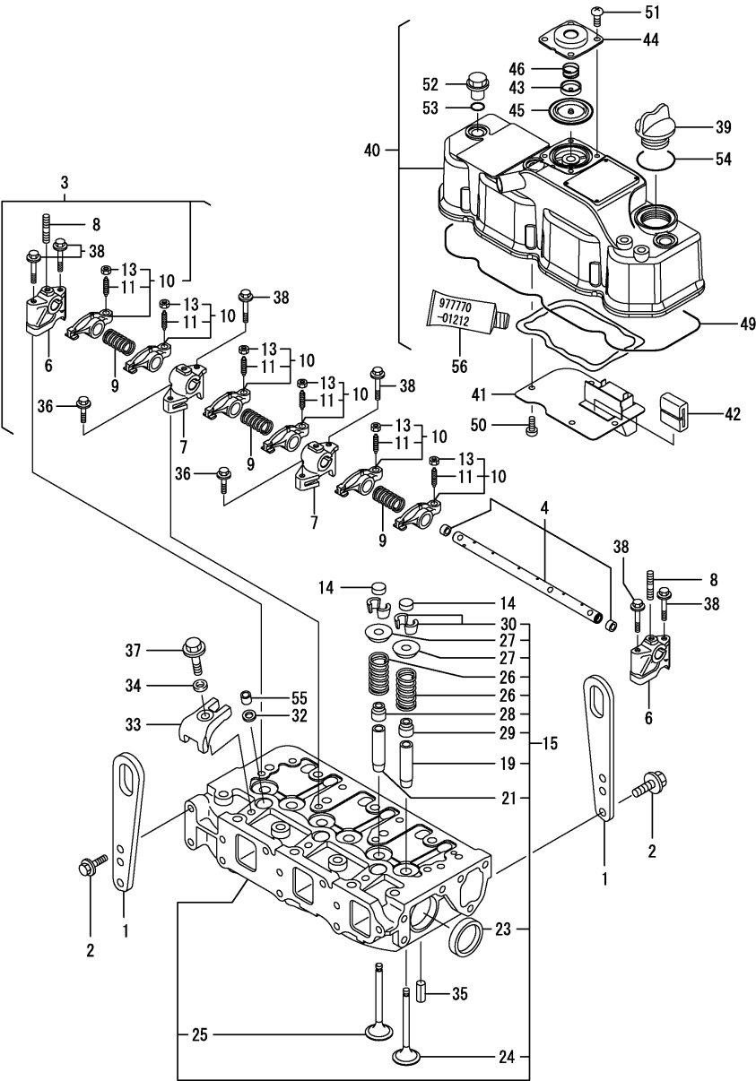
Fig.4.CYLINDER HEAD & BONNET
