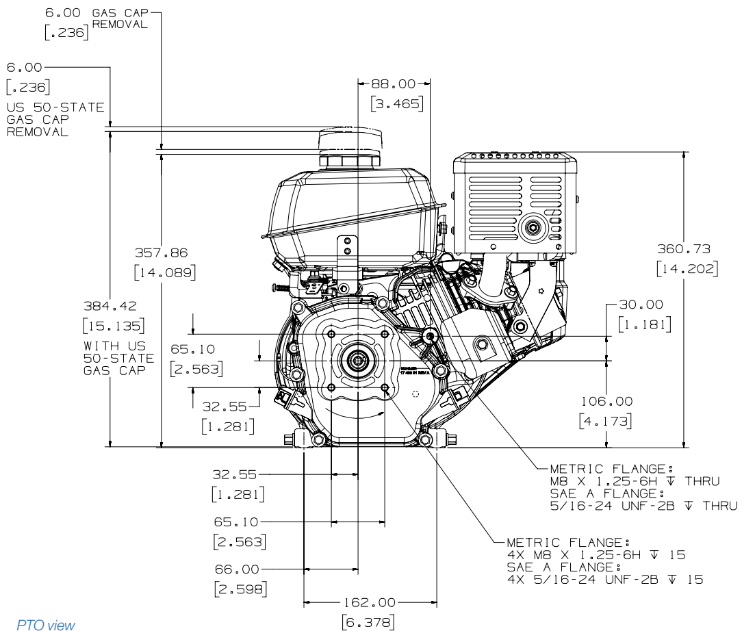
PTO view
