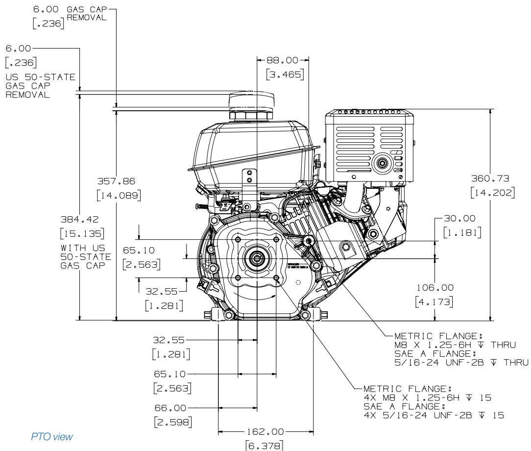
Top view
