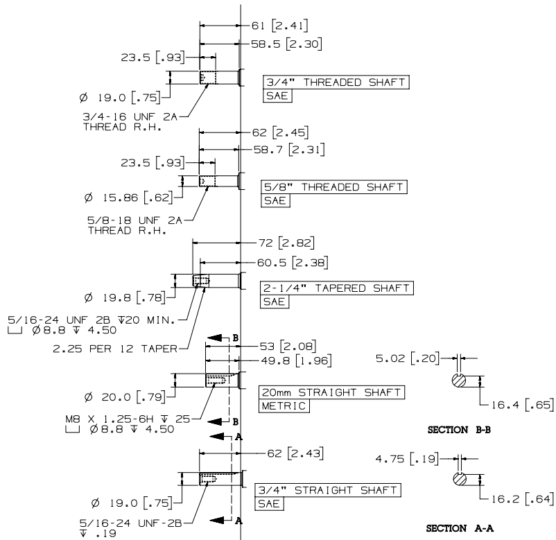
Shaft variations
