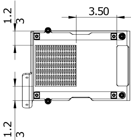
RIGHT HAND DRIVE CONTROLLER
