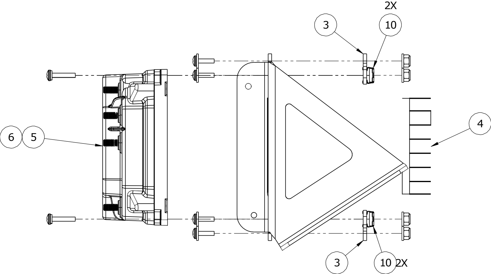
RIGHT HAND DRIVE CONTROLLER
