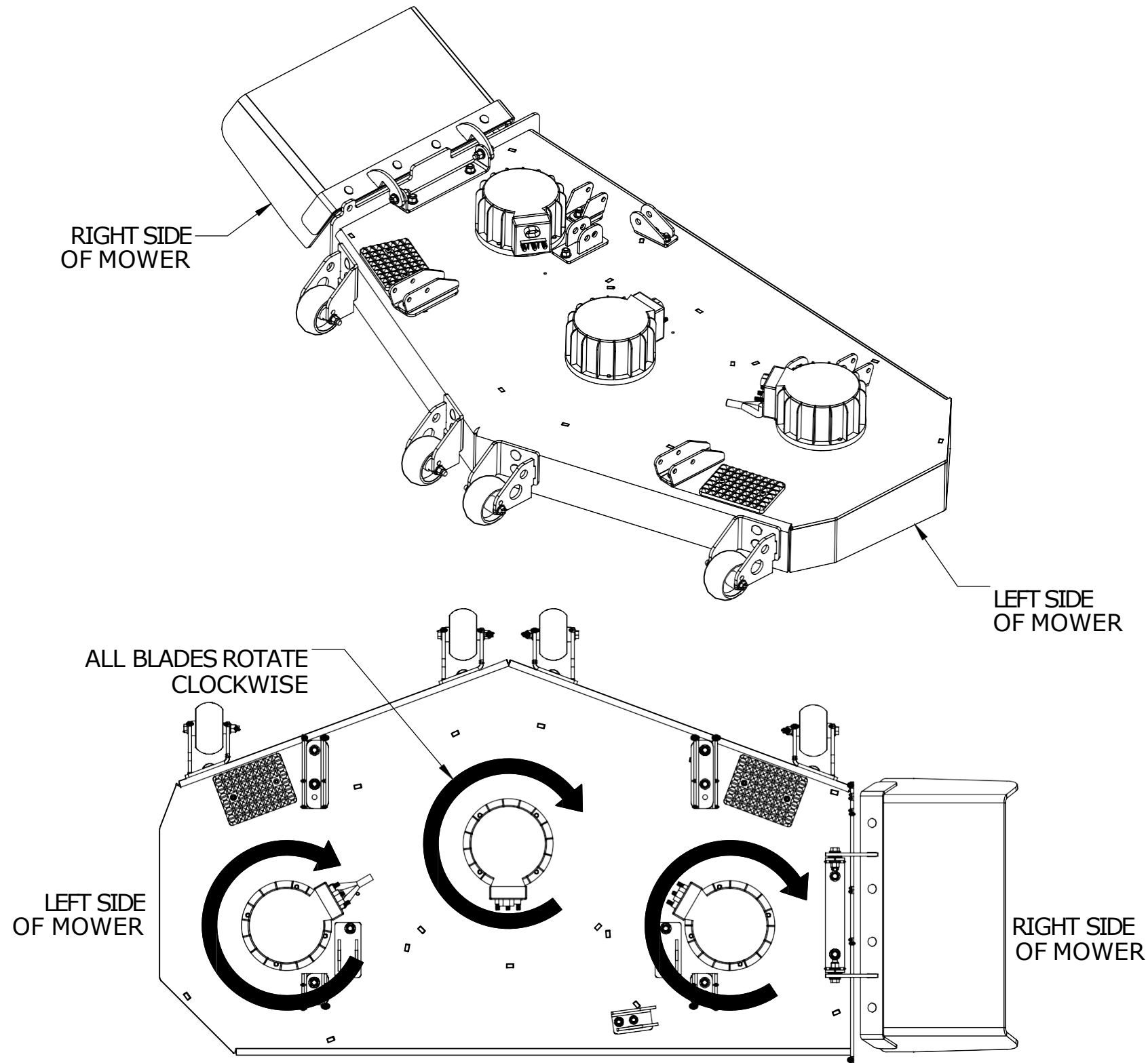
VIEW FROM TOP OF DECK
