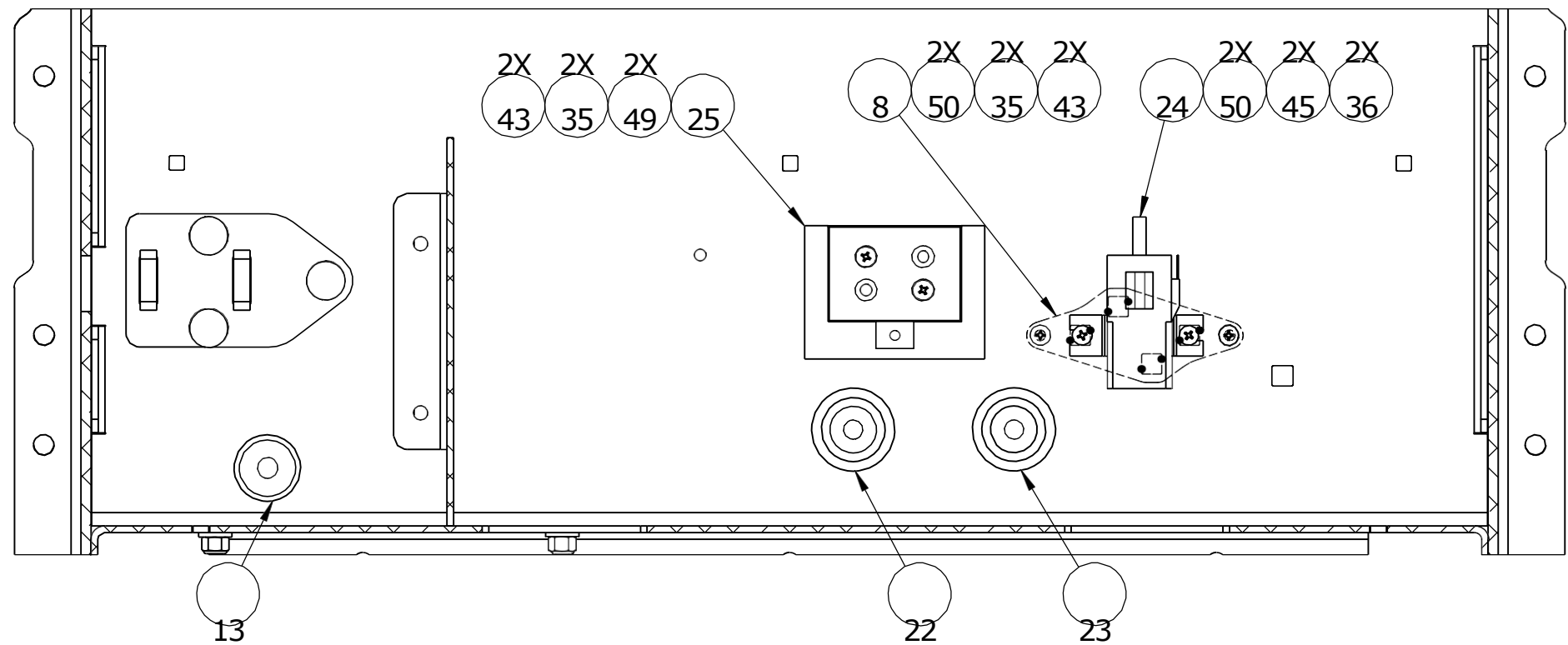
VIEW FROM INSIDE ELECTRICAL COMPARTMENT (UNDER SEAT)
