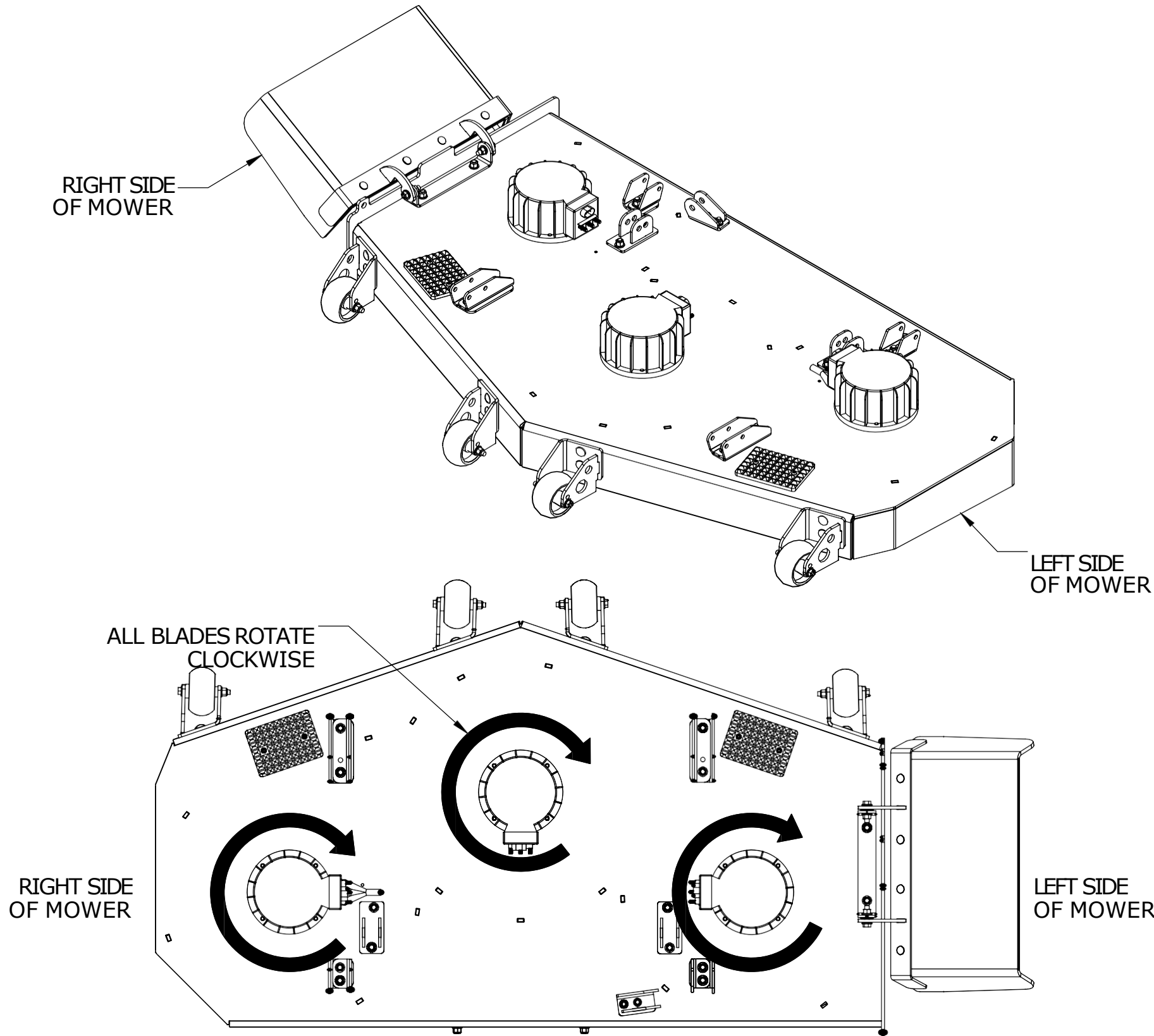
VIEW FROM TOP OF DECK
