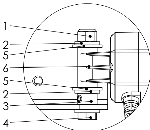
DETAIL B SCALE 1 : 1.5
